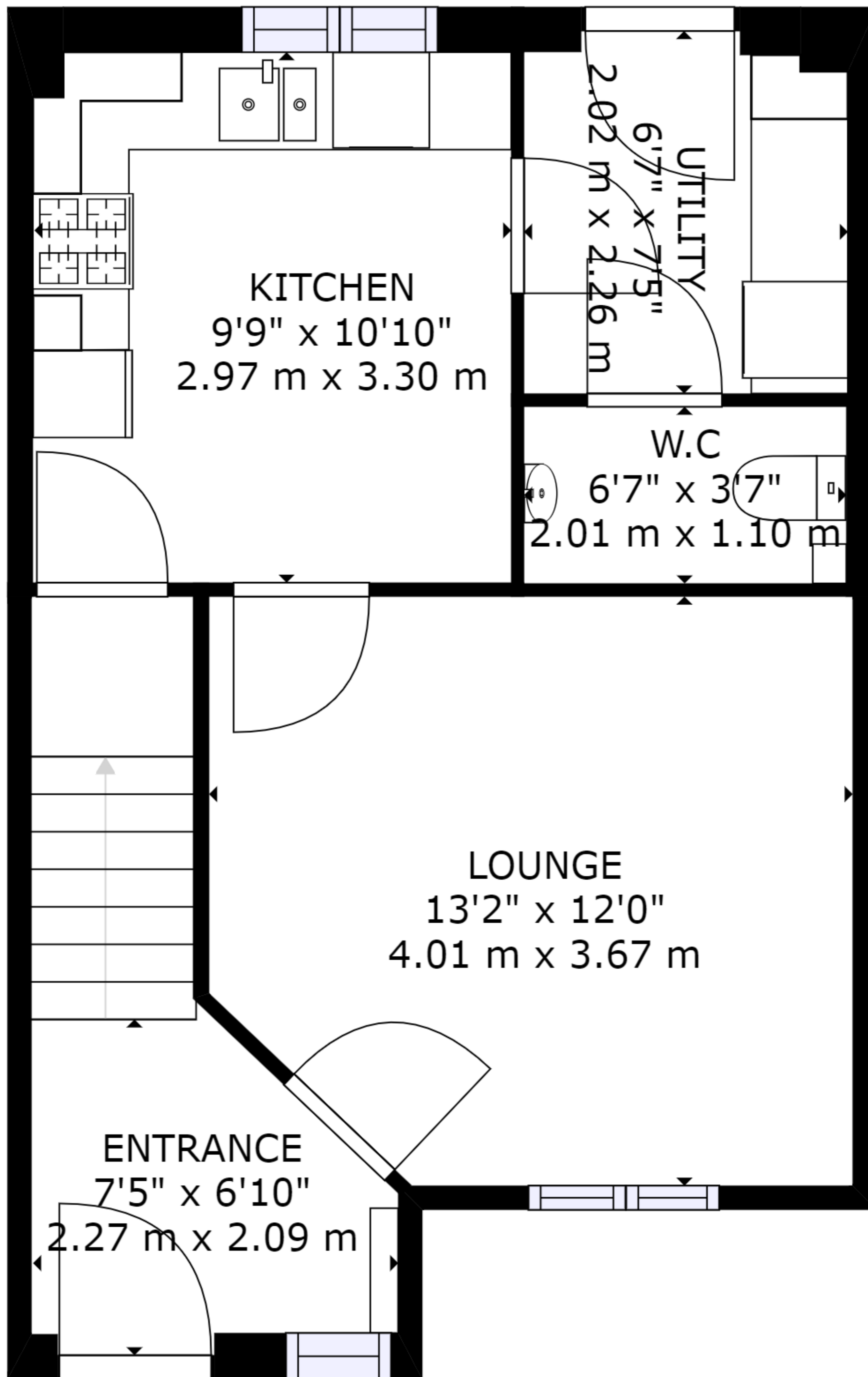
FLOOR 1
